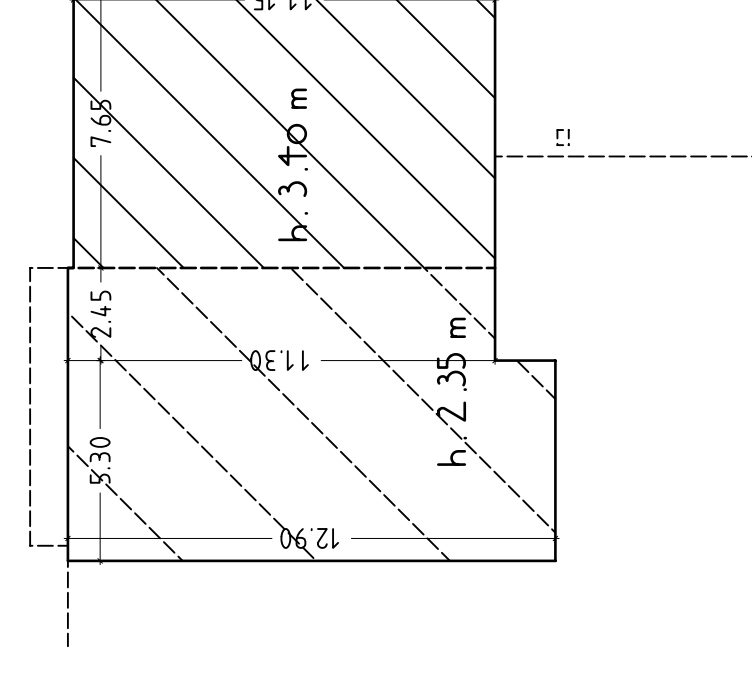
PIANO SEMINTERRATO SIP = 65,30 m 2
